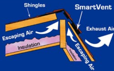
Dormer Peak
