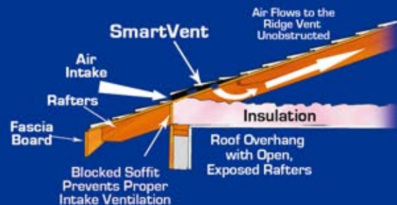
Mid-Roof Application
